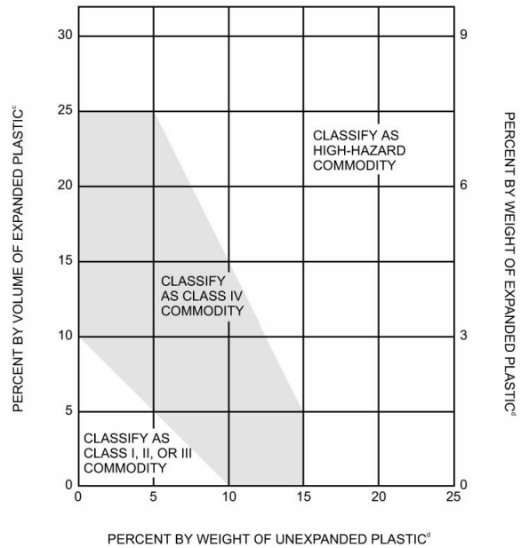
Figure 2303.7.4 Mixed Commodities
